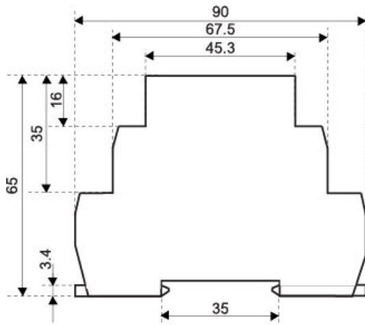
1-MODULE DESIGN
