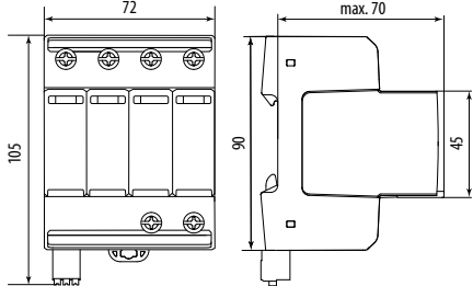
ETITEC ML T123 300/12,5 (4+0) RC/ ... (3+1) RC
