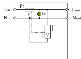
ETITEC LP2 IP20
