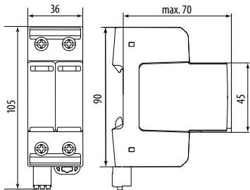
ETITEC ML T123 300/12,5 (2+0) RC/ ... (1+1) RC
